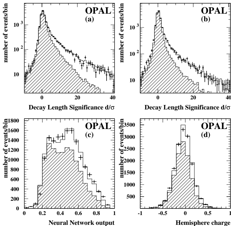
Fig. 2. Distributions of the different tag-variables used in the flavour separation. Shown are the data distribution after background subtraction ( points with error bars ), the equivalent Monte Carlo distribution for all candidates ( open histogram ) and the predicted charm component ( hatched histogram ). Shown are the a decay length significance in the jet with the exclusive D^{*+} candidate; b decay length significance in the jet opposite the exclusive D^{*+} candidate; c distribution of the neural network based on jet-shape variables, and d distribution of the hemisphere charge.
