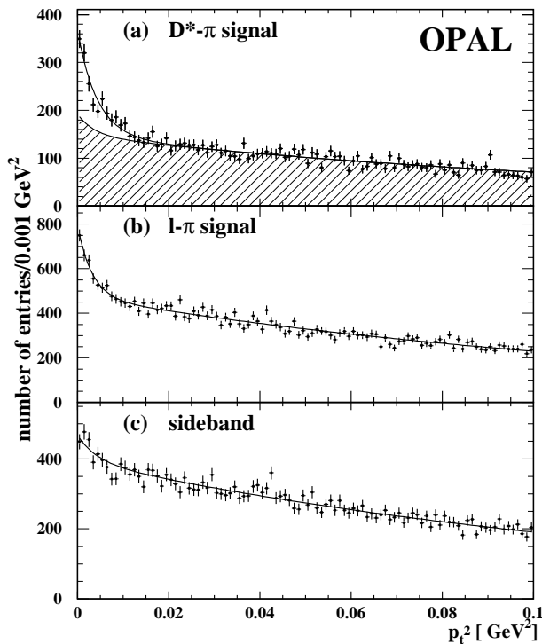
Fig. 5. Spectrum of the squared transverse momentum of double tagged candidates after applying all cuts of the a signal candidates, reconstructed with opposite charges in both jets. The non-charm component is indicated by the hatched area ; b lepton-tagged candidates. The points are the data and the lines the results of the fit; c background candidates, reconstructed in \Delta M sidebands
