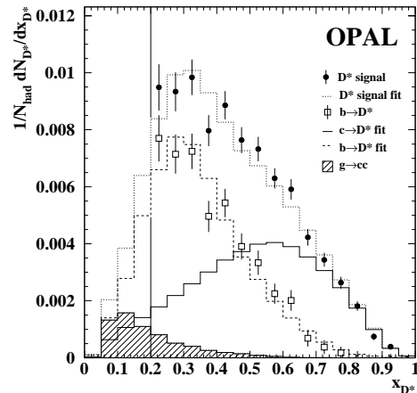
Fig. 4. Efficiency corrected yield of D^{*+} mesons as a function of the scaled energy x_{D^{*+}} , 1/N_{\text{had}}dN_{D^{*+}}/dx_{D^{*+}} , for all candidates ( filled points with error bars ) reconstructed in the decay D^{*+} \rightarrow D^0\pi^+ , D^0 \rightarrow K^-\pi^+ , and the charm component after flavour separation ( solid line ). The open points are the bottom component, and the dashed line represents the result of the fit. Also shown is the predicted contribution from gluon splitting events ( hatched area ). The reconstruction is only done for x_{D^{*+}} > 0.2 , as indicated by the solid vertical line
