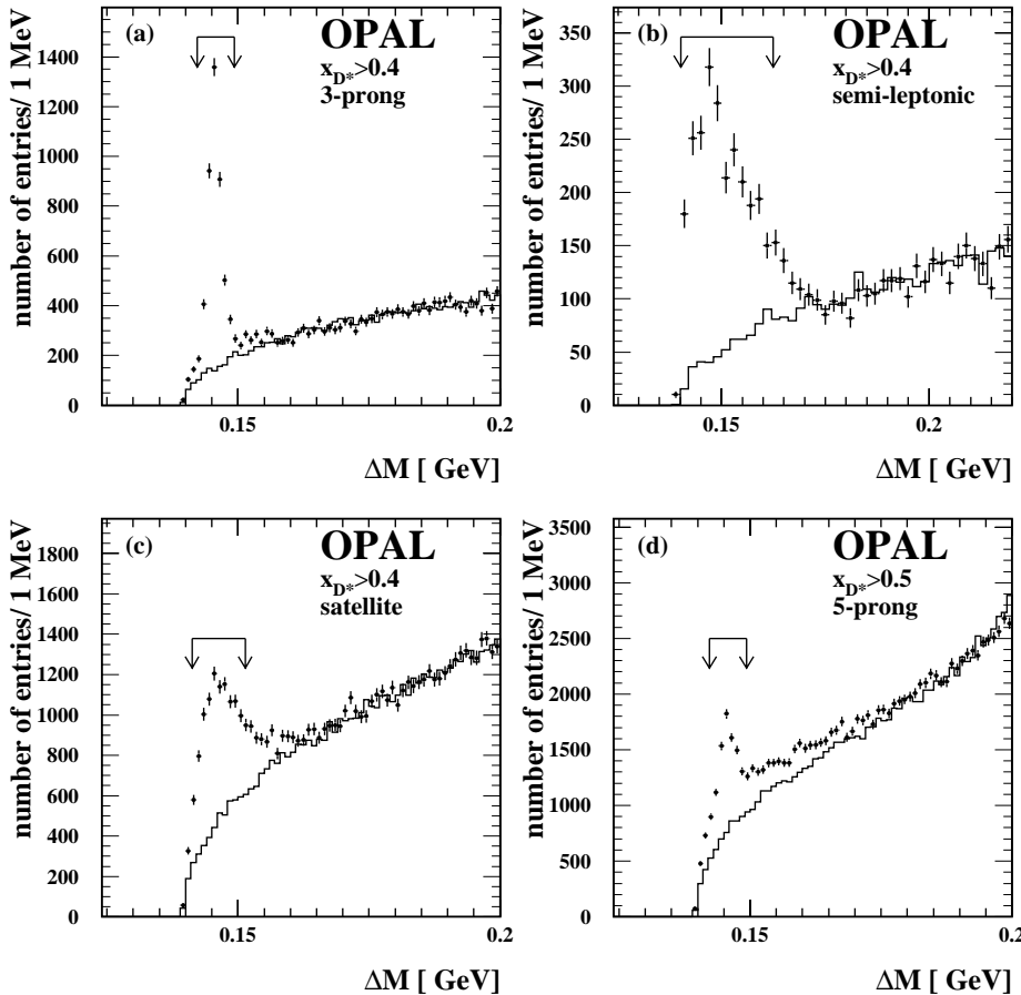
Fig. 1. Distributions of the difference \Delta M = M_* - M_0 reconstructed in the four different D^{*+} channels. The arrows indicate the selected signal region. a 3-prong decay mode, b the two semileptonic modes combined, c the satellite decay mode, and d the 5-prong decay mode. The points with error bars are the signal candidates. Superimposed in each case (line histogram) are the background estimator distributions, normalised to the upper sidebands in \Delta M
