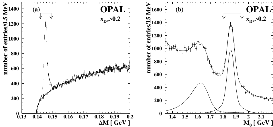
Fig. 3. a Distribution of the mass difference \Delta M = M_* - M_0 reconstructed in the decay D^{*+} \rightarrow D^0\pi^+ , D^0 \rightarrow K^-\pi^+ . Superimposed is the background distribution obtained from the background estimator discussed in the text, and the result of the fit to this background estimator. The arrows indicate the selected signal region. b M_0 spectrum of D^{*+} candidates, with M_0 cut removed, and an additional \Delta M cut applied. Shown are the data ( points with error bars ), the result of the fit as described in the text, and the two components from satellite and from fully reconstructed D^{*+} mesons, as obtained in the fit. The arrows indicate the selected signal region
